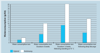
WATER CONSUMPTION: HYBRID - ANTIMONY
