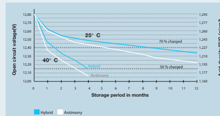
SELF-DISCHARGE: HYBRID - ANTIMONY
